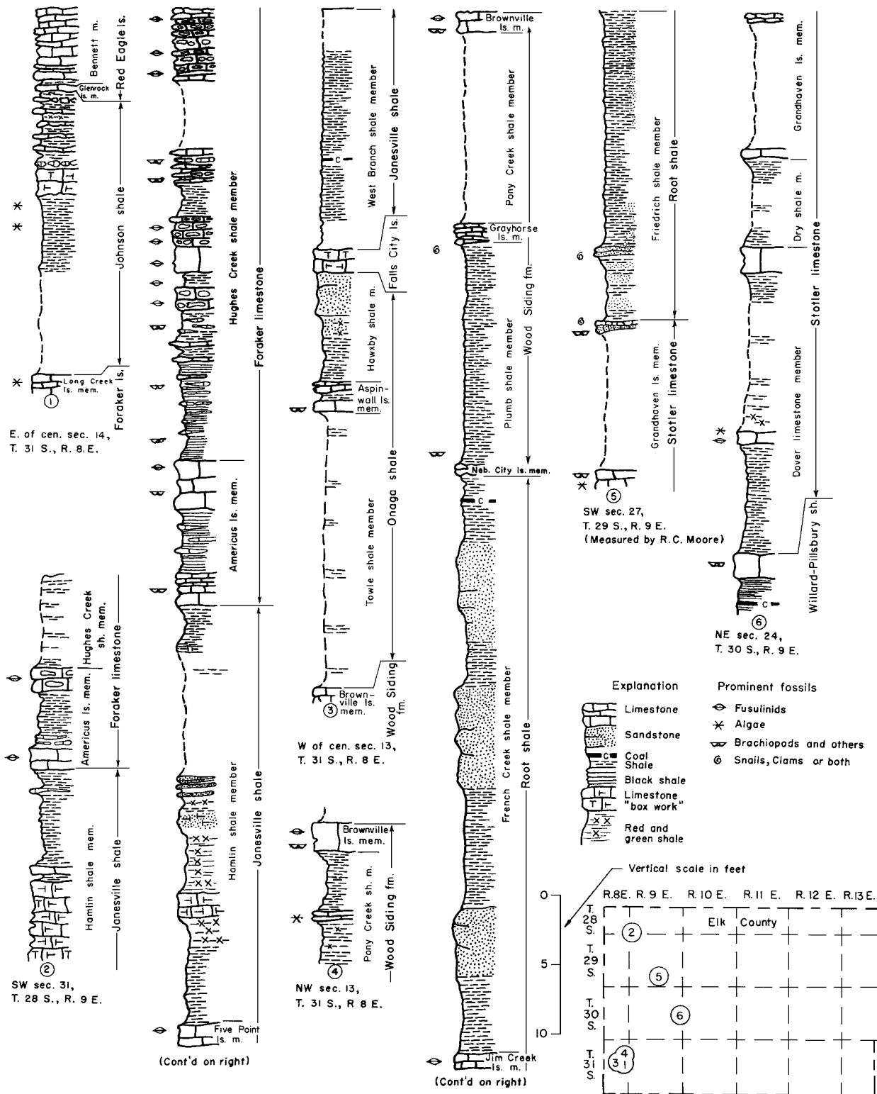
Figure 3— Diagrammatic representation of outcropping lower Wolfcampian (Permian) and upper Virgilian (Pennsylvanian) rocks.
