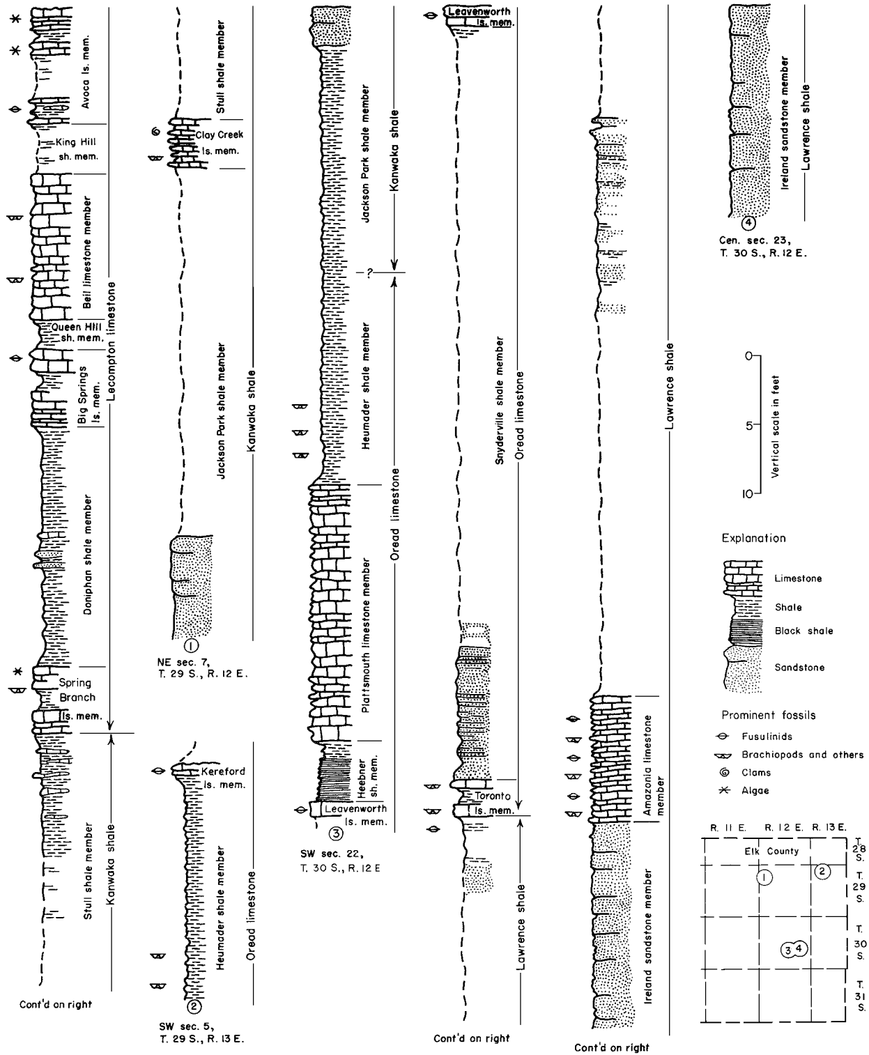
Figure 6 – Diagrammatic representation of outcropping lower Virgilian (Pennsylvanian) rocks.
