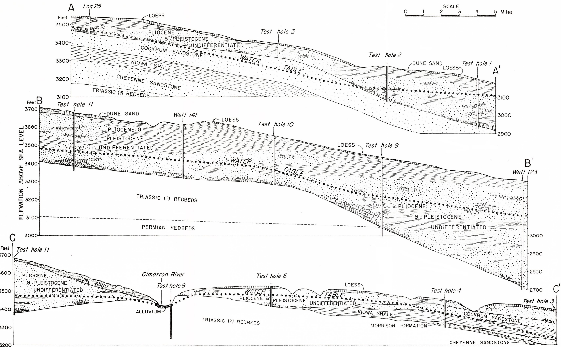
PLATE 6. A, East-west geologic profile across the northern part of Morton county (line A-A', fig. 2). B, East-west geologic profile across the southern part of Morton county (line B-B', fig. 2). C, North-south geologic profile across the western part of Morton county (line C-C', fig. 2).
