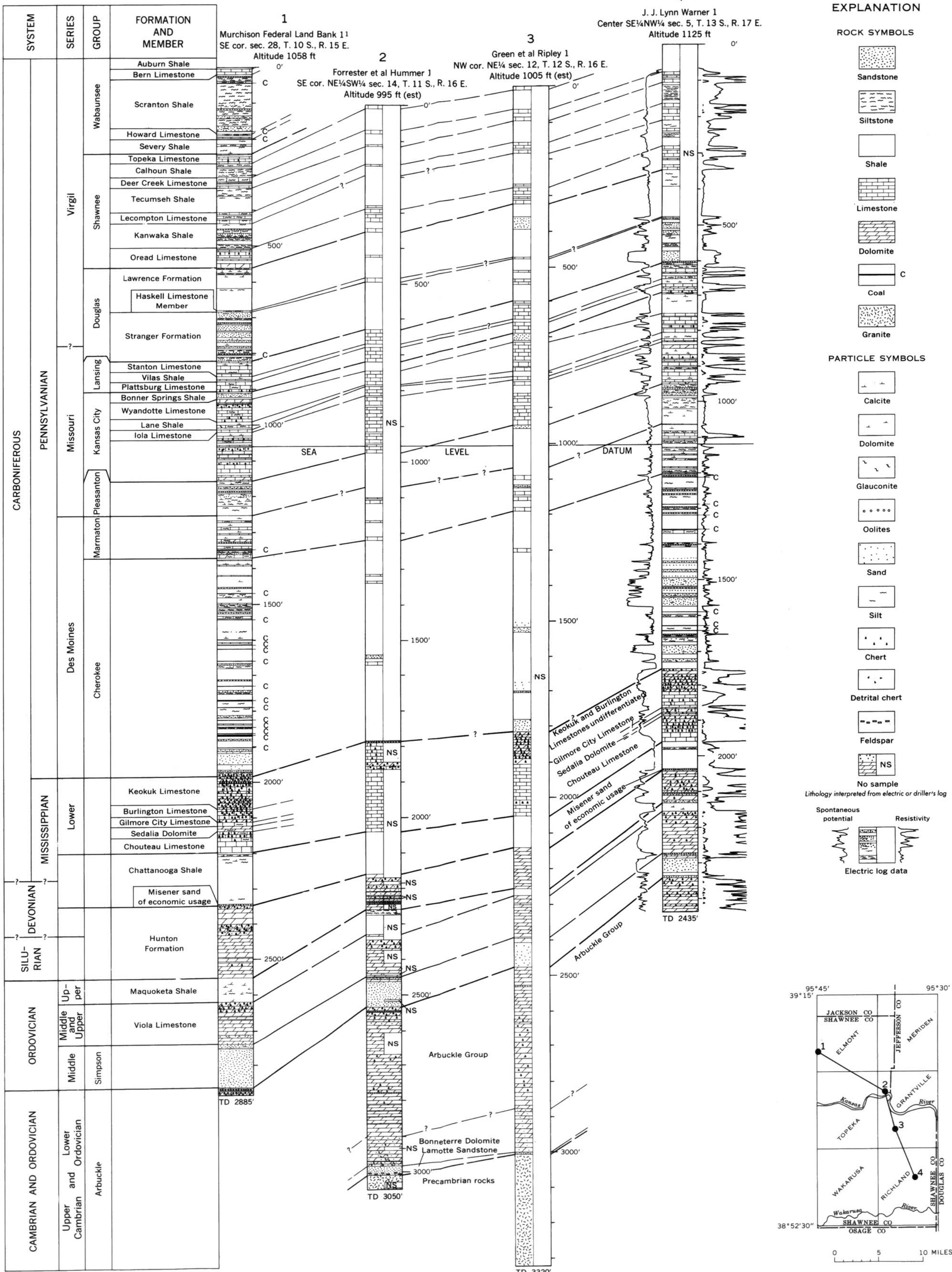
SUBSURFACE SECTIONS IN EASTERN SHAWNEE COUNTY, KANSAS
