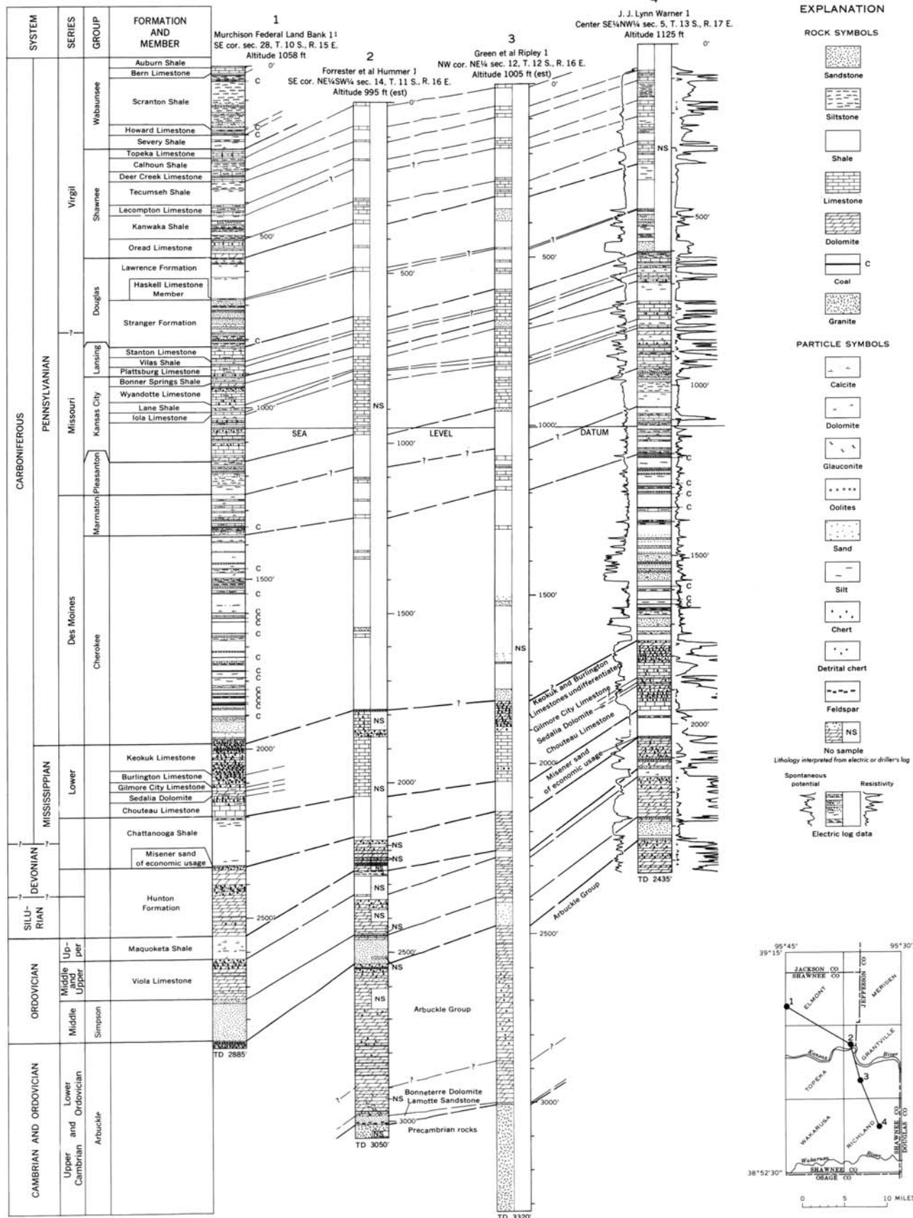
SUBSURFACE SECTIONS IN EASTERN SHAWNEE COUNTY, KANSAS
