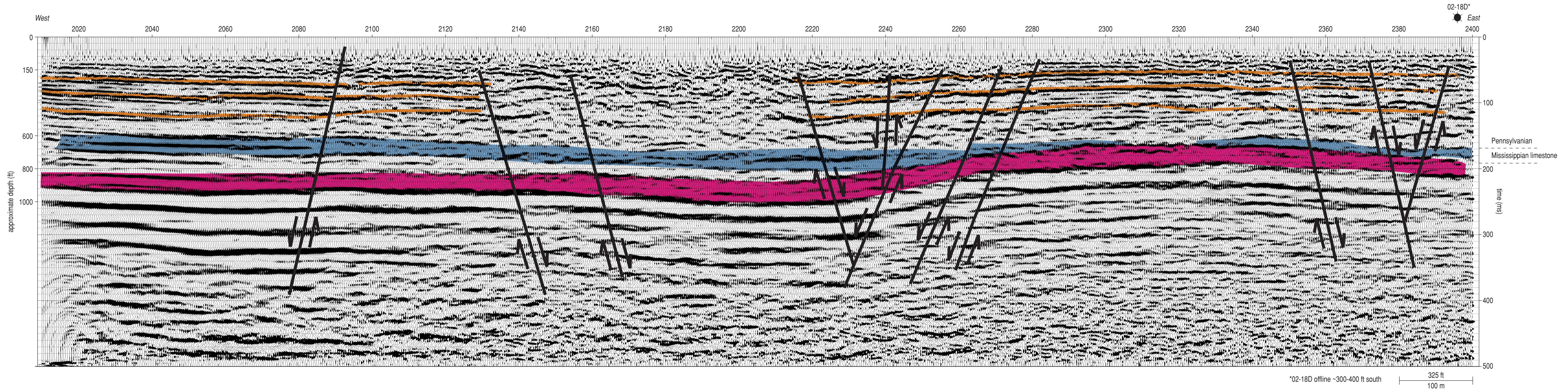
Figure 22. Interpreted CMP-stacked section of line 2 (north property line).
