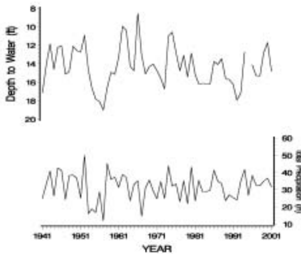
FIGURE 7. Depth to water in Sedgwick County, well 25S-01W-14-DDD-01 [alluvial aquifer], and precipitation at Mount Hope (station 14553908).
