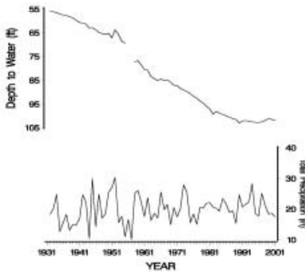
FIGURE 6. Depth to water in Scott County, well 20S-33W-09-BBB-01 [128 ft (39.0 m) deep; High Plains aquifer], and precipitation at Scott City (station 14727104).
