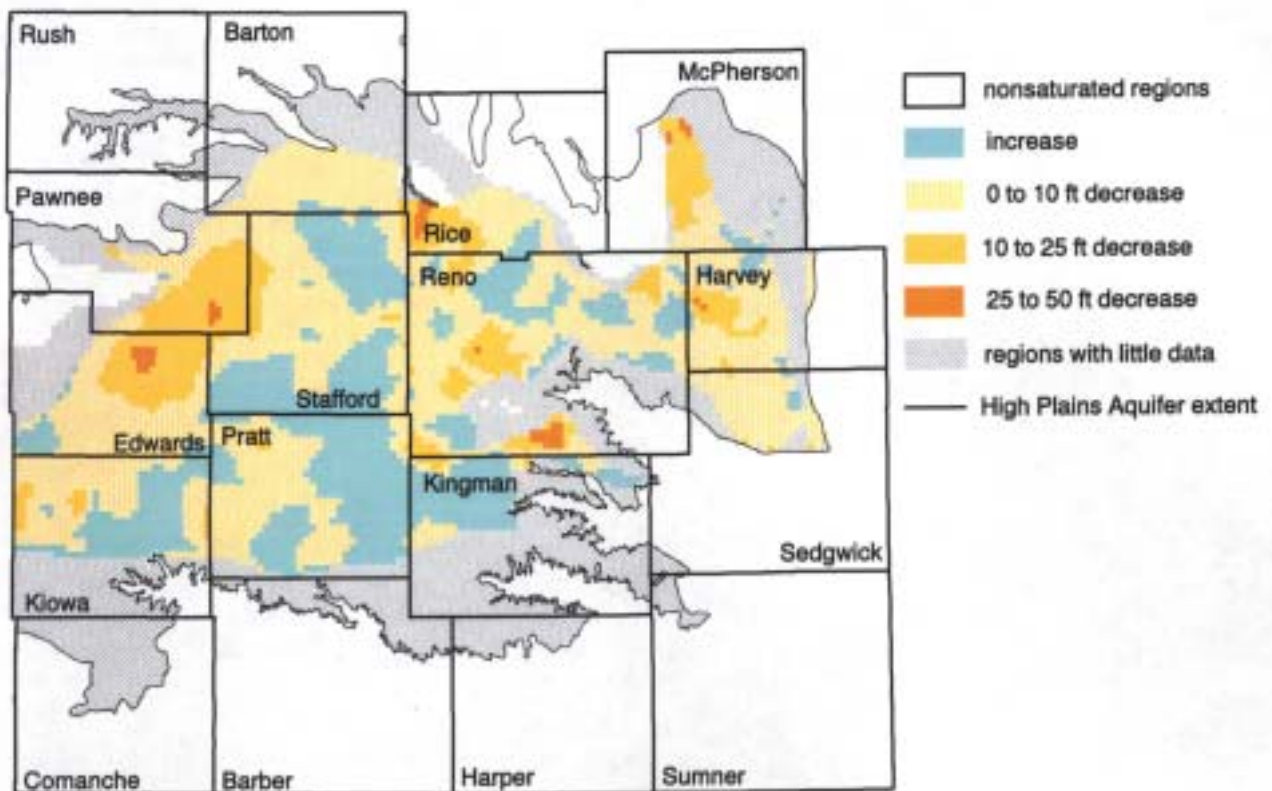
FIGURE 12A. Ground-water changes in the area of the High Plains aquifer in Region V, south-central Kansas. See fig. 9 for adjacent areas to the west. Generalized water-level changes (ft), predevelopment to 2001.
