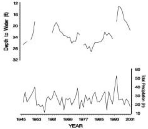
FIGURE 4. Depth to water in Hamilton County, well 23S-43W-21-ABA-01 [29 ft (8.8 m) deep; alluvial aquifer], and precipitation at Syracuse (station 14803807).
