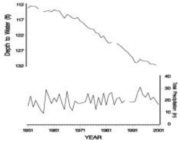
FIGURE 8. Depth to water in Thomas County, well 08S-34W-01-BAC-01 [175 ft (53.3 m) deep; High Plains aquifer], and precipitation at Colby 1 SW (station 14169901).
