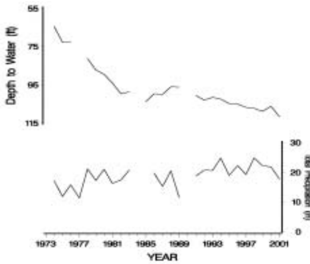
FIGURE 3. Depth to water in Finney County, well 24S-33W-28-DAA-01 [350 ft (107 m) deep; High Plains aquifer], and precipitation at Garden City Experimental Station (station 14298007).
