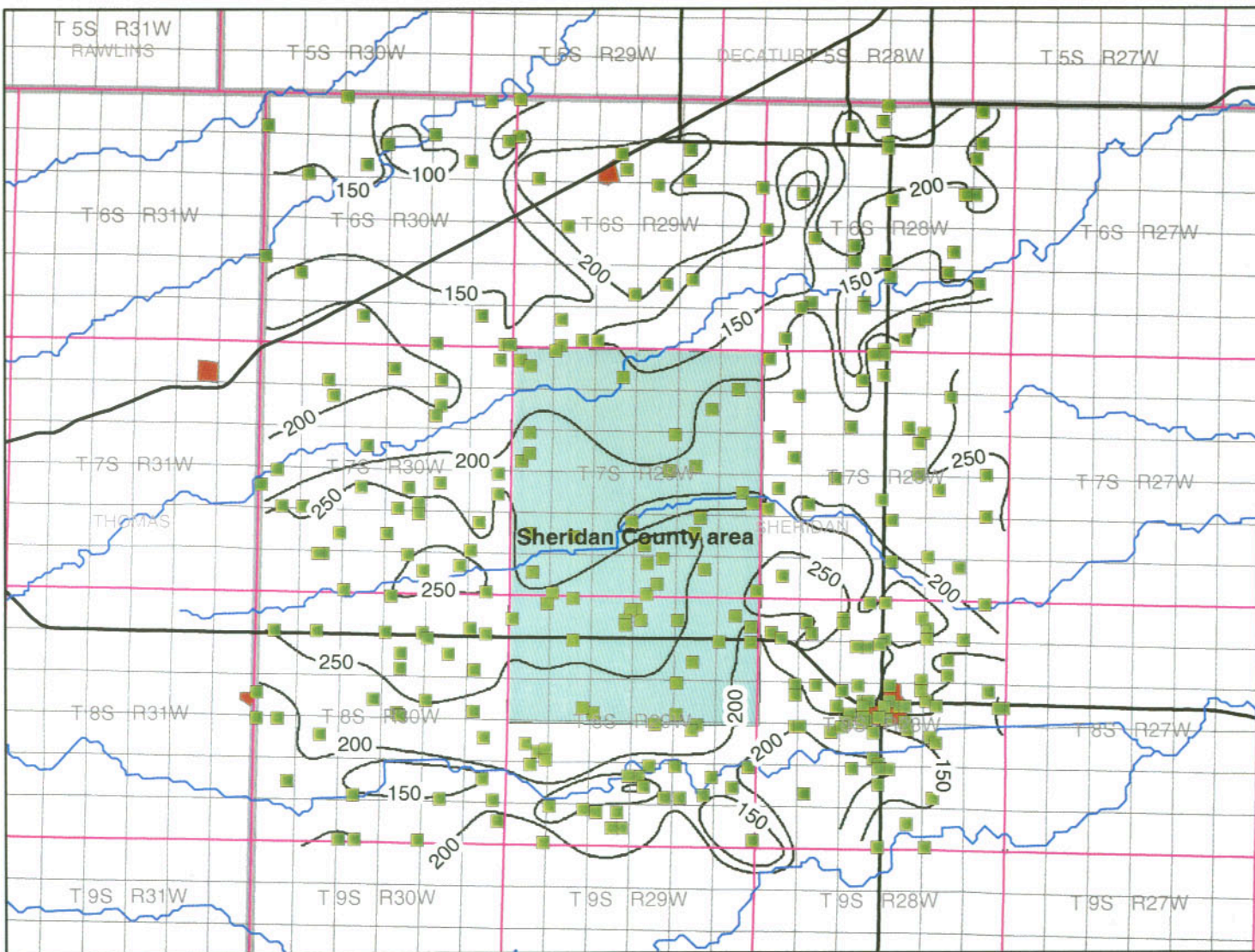
Figure 20 The combined Ogallala Formation – undifferentiated Quaternary thickness in the Sheridan County study area Drawn by Date File Name Projection Scale grh 02/10/03 Fig 20 Total thickness.mxd UTM Zone 14 NAD 1983 1:250,000
