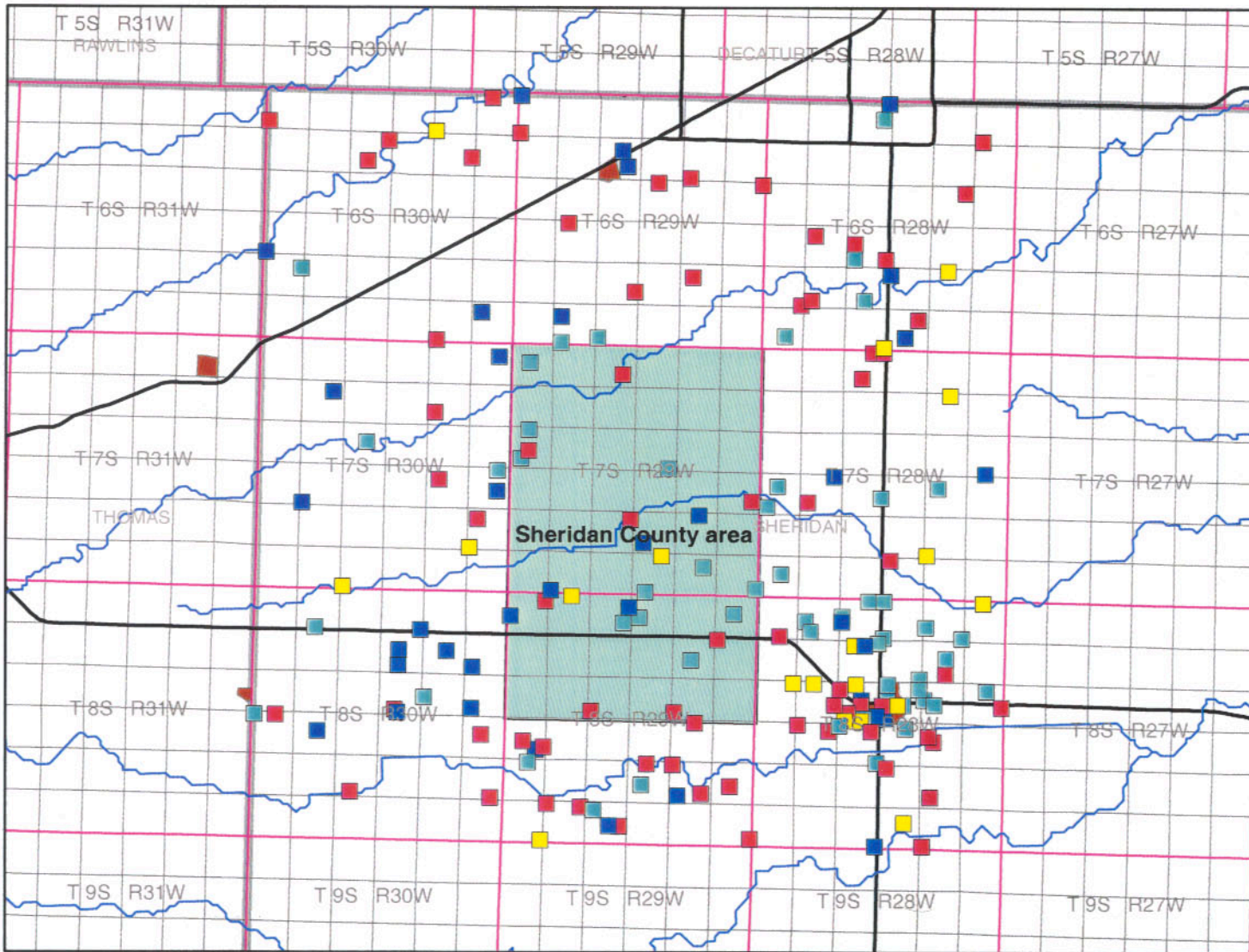
Figure 29 30 The sand and gravel fraction percentiles in the lower half of the combined Ogallala Formation – undifferentiated Quaternary, Sheridan County study area. Drawn by Date File Name Projection Scale grh 02/10/03 Fig 29 Sand plus gravel frac L.mxd UTM Zone 14 NAD 1983 1:250,000
