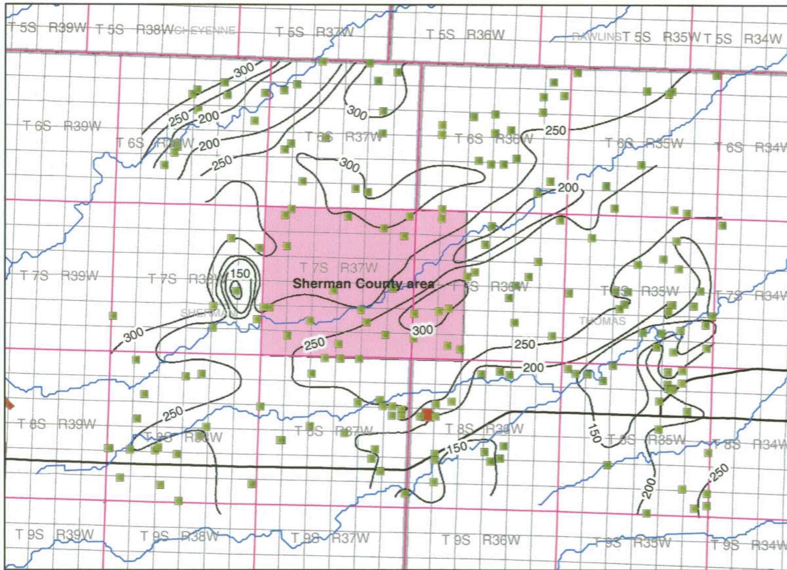
FIGURE 6 The combined Ogallala Formation – undifferentiated Quaternary thickness in the Sherman County study area. Drawn by Date File Name Projection Scale grh 02/10/03 Fig 6 Total thickness.mxd UTM Zone 14 NAD 1983 1:250,000
