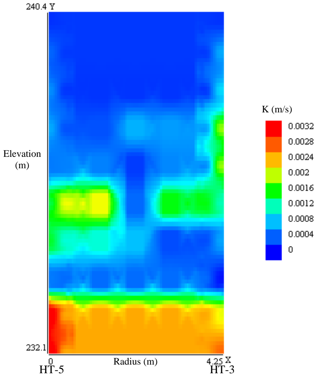
Figure 51: Interwell K values from constrained SVD analysis with HT-5 as the source well and HT-3 as the receiver well ( S_s = 1.5 \times 10^{-5} ).
