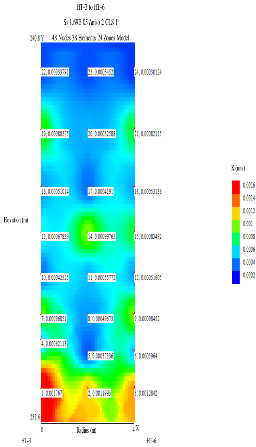
Figure 74. K values from constrained SVD analysis of 784 rays at HT-3 (receiver) to HT-6 (source). K values range from 0.0003 to 0.0018 m/sec (0.0010 to 0.0058 ft/sec).
