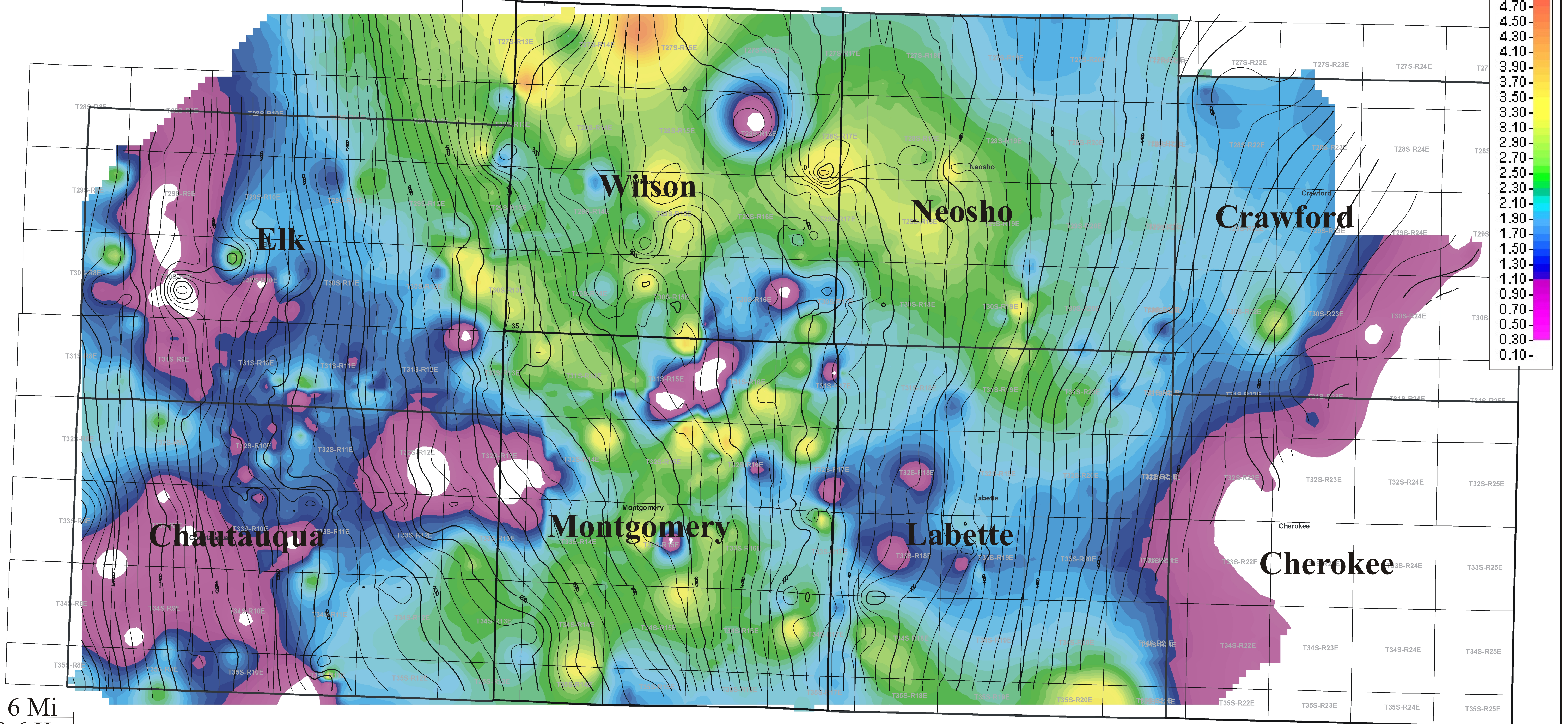
Isopach of Aw coal (colors) overlain with contours on bottom Aw structure (isopach CI: 0.10ft; structure CI: 25ft)
