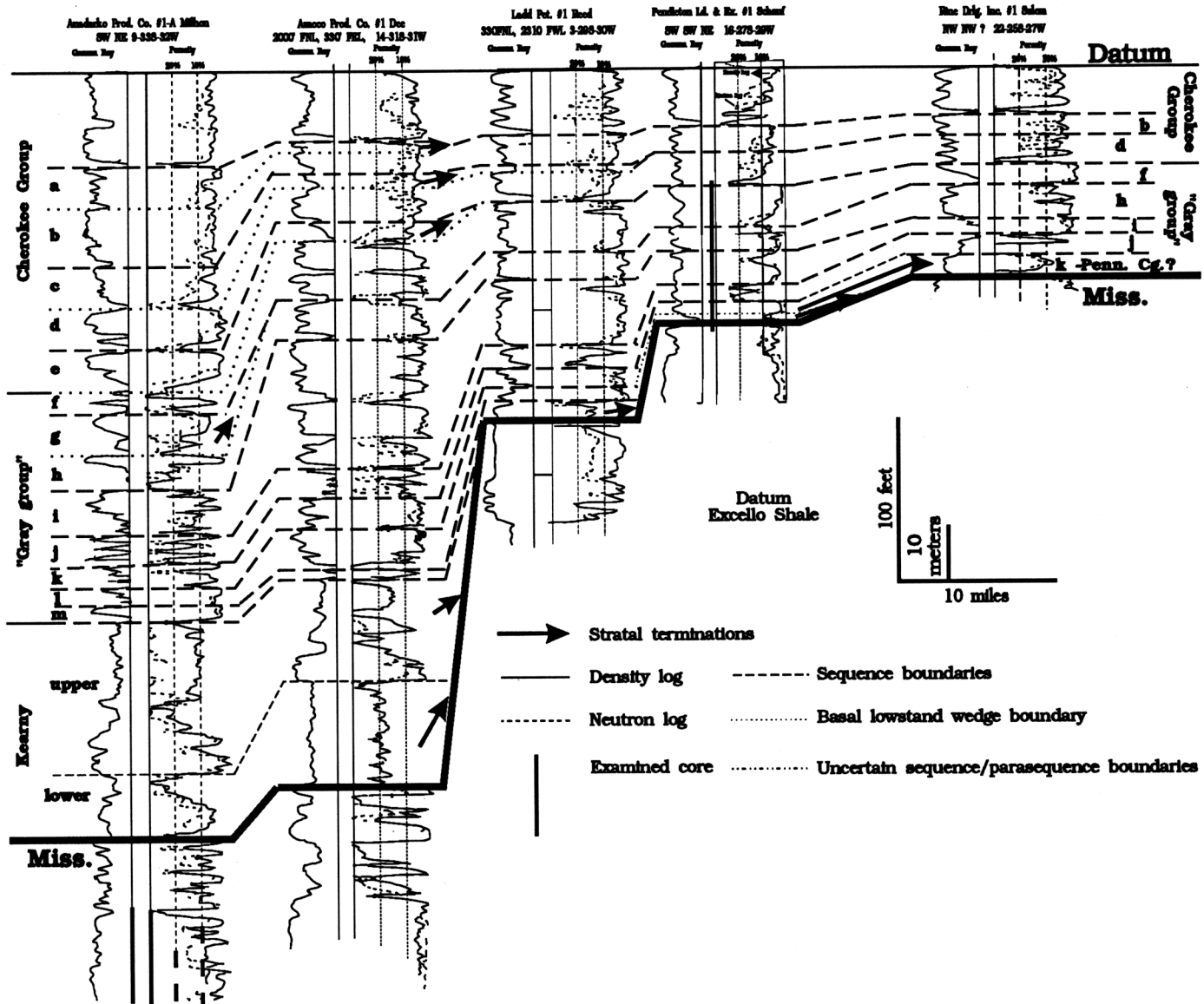
FIGURE 4—CROSS SECTION H-H' FROM "GRAY GROUP" REFERENCE SECTION located in the Anadarko Production Co. #1-A Milhon through "Gray group" type section located in the PL&E #1 Schaaf.
