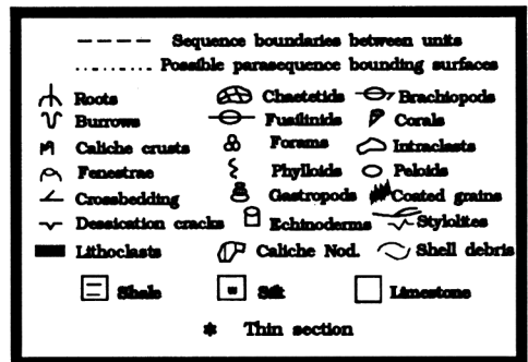
FIGURE 7—CORE DESCRIPTION OF TYPE SECTION OF "GRAY GROUP" ROCKS IN Pendleton Land & Exploration #1 Schauf, sec. 16, T. 27 S., R. 29 W., Gray County, Kansas.
