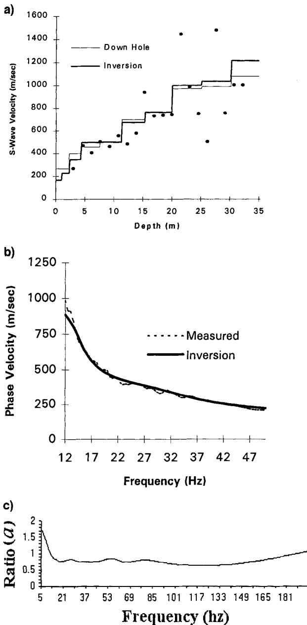
FIG. 5. Inversion results from a field test of (a) a v_s profile and (b) the corresponding dispersion curve in comparison with a downhole v_s profile and measured dispersion curve. Dots in the displayed v_s profile in (a) represent the data points actually measured during the downhole survey. The downhole profile was recalculated from these data according to the thickness model used in the inversion process. (c) The ratio a in equation (7) that was used during construction of the initial v_s profile.
