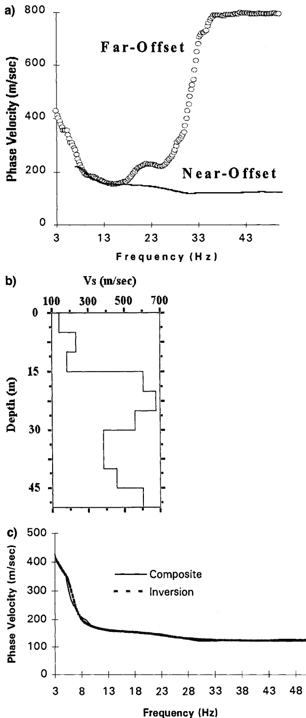
FIG. 7. (a) Dispersion curves obtained by processing near-offset (4–30 m) traces and far-offset (30–60 m) traces of the record in Figure 6a separately. (b) A v_s profile obtained from the inversion of a composite dispersion curve created by integrating the two curves. (c) The composite dispersion curve in comparison with the dispersion curve corresponding to the inverted v_s profile in (b).
