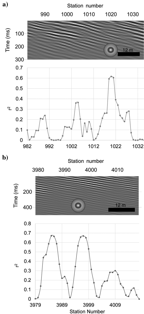
Figure 7. (a) BASW image and the correlation diagram optimized using amplitude thresholding at the Yuma tunnel site set at a different lateral location and collected with a 29.3 m SO (versus Figure 6). (b) BASW image and amplitude-threshold correlation diagram for a clandestine tunnel in Afghanistan. Again, tunnel locations are detailed by the bulls' eyes.
