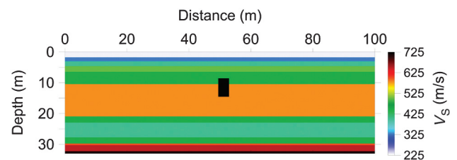
Figure 3. The V_S model for the Yuma site, with exaggerated tunnel not to scale (black rectangle).
