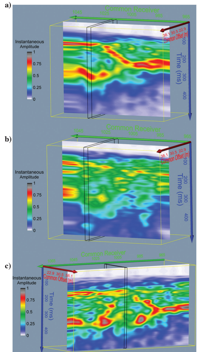
Figure 10. Amplitude cube comparing the (a) full-wavefield and (b) primarily backscattered energy. (c) At a farther-offset slice with integrated forward- and reverse-source rolls, we retrieve a semisymmetrical event emanating from the tunnel location.
