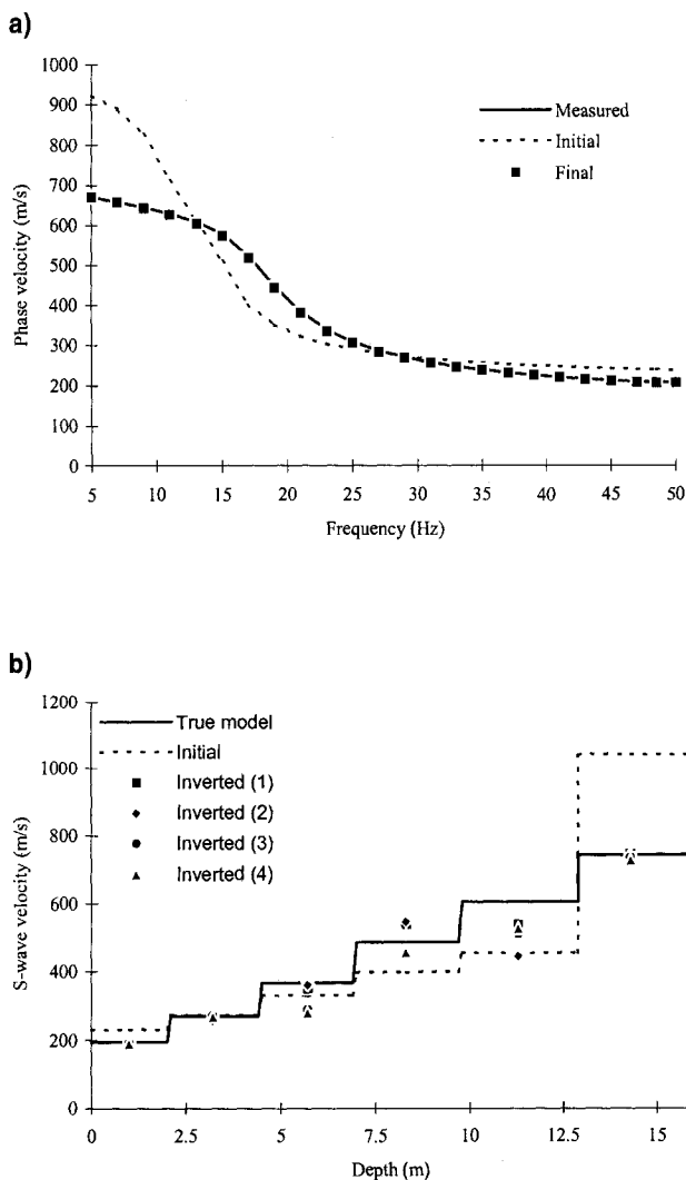
FIG. 4. Inversion results of multilayer examples. Labels on dispersion curves (a) and S -wave velocity profiles (b) have the same meaning as labels in Figure 3. The true model (b) is listed in Table 1. The initial model (b) except for the S -wave velocity of the half-space shown by the dashed line was calculated based on equation (6). Four inverted models (b) marked by different symbols were the final models of four cases from our inverse procedure. One of every two phase velocities attributed to the inverted model is shown by squares (a).
