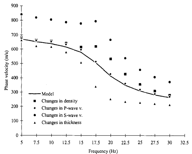
FIG. 2. Contributions to Rayleigh-wave phase velocity by 25% changes in each earth model parameter (Table 1). The solid line is Rayleigh-wave phase velocity attributed to the earth model listed in Table 1. Squares represent Rayleigh-wave phase velocities after 25% changes in density; diamonds represent Rayleigh-wave phase velocities after 25% changes in P -wave velocity, etc.
