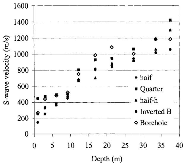
FIG. 8. Effect of the number of data points on inversion results. The solid diamonds indicate the inversion results from data points from 15 to 47 Hz (33 points); solid squares, 15 to 31 Hz (17 points); solid triangles, 15 to 47 Hz with an interval of 2 Hz (17 points); and solid circles, 15 to 80 Hz.
