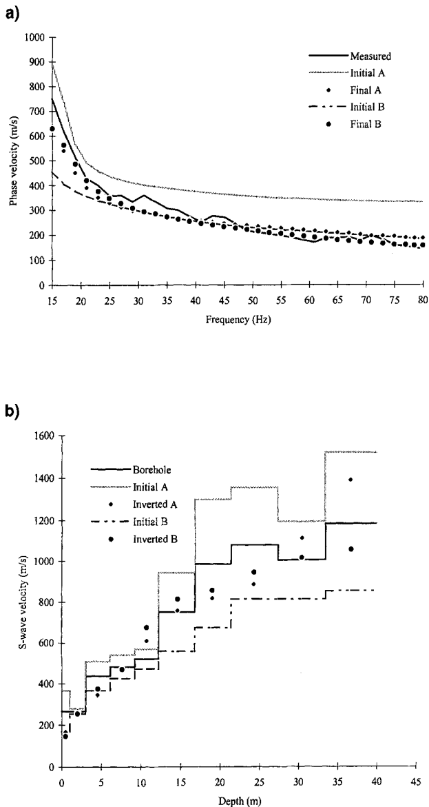
FIG. 6. Inverse results of the real example. Labels on dispersion curves (a) and S -wave velocity profiles (b) have the same meaning as in labels Figure 4, except that the dispersion curve labeled measured (a) is real data extracted from filed data (Figure 5) by CCSAS techniques (Park et al., 1998). Initial B model (b) was calculated from the measured data in (a) based on equation (6). Borehole (b) was S -wave velocities derived from the three-component seismic borehole survey. Initial A and Initial B models (b) are symmetrical to the borehole values. Both initial models converge to the model determined by borehole data. One of every two phase velocities attributed to the inverted models is shown by diamonds and dots (a).
