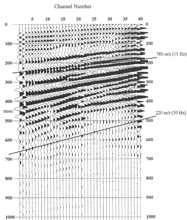
FIG. 5. The field data acquired near the Kansas Geological Survey during the winter of 1995. Forty groups of 10-Hz geophones were spread 1 m apart. An IVI MiniVib was used as the energy source and was located 27 m away from the right side of the geophone spread. Two linear events are velocities of dispersive ground roll at frequencies of approximately 15 and 50 Hz.
